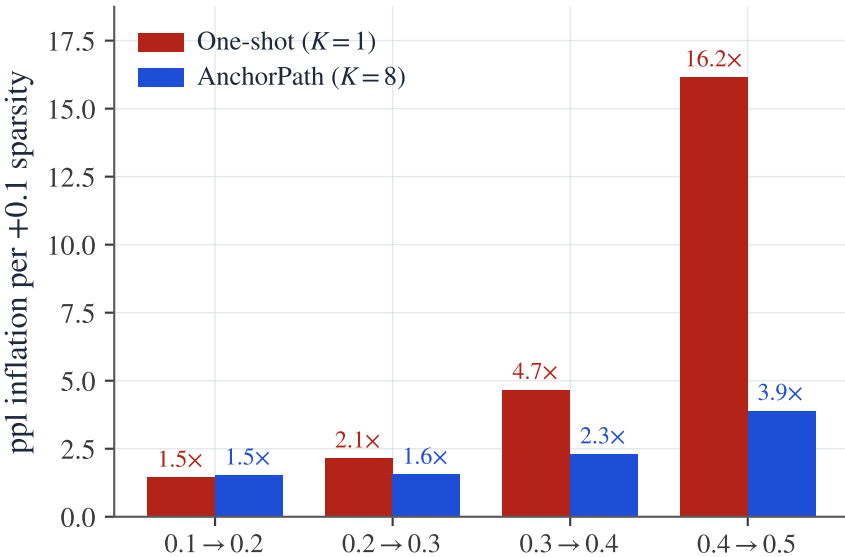
(a) Collapse is super-exponential
